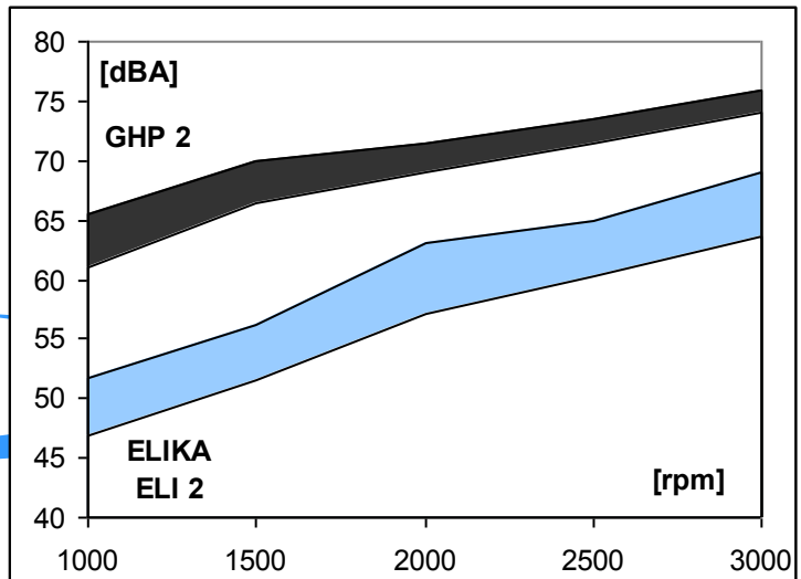
Noise pump comparison [dBA] Marzocchi GHP2 – ELIKA ELI 2, same displacement 17.8 cm 3 /rev, pressure from 10 to 250 bar.
