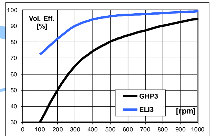
Comparison of volumetric efficiency at low rotation speed, Pm=200 bar Marzocchi GHP 3 – ELIKA ELI 3, displacement 26.3 cm 3 /rev.
